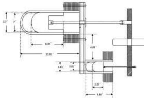
Fig 3.7 CAD diagram of calculated engine parameters
