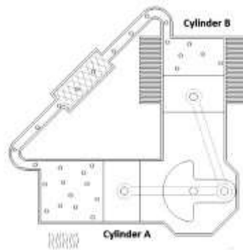
Fig 3.1 Stirling Cycle
