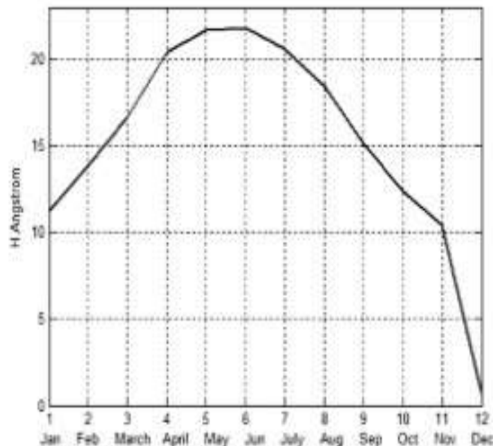
Fig 1: Daily global solar radiation of Multan
