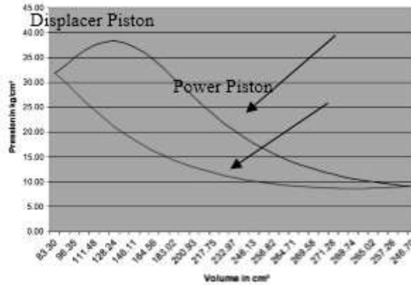
Fig 3.6 Pressure Volume Diagram
