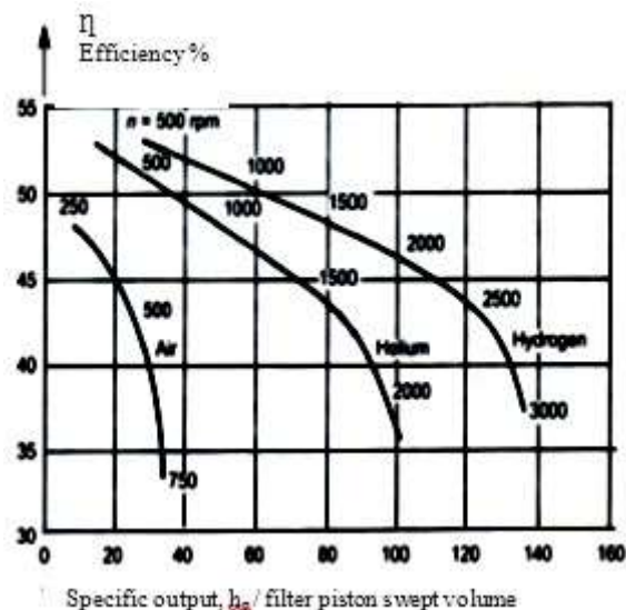
Fig 3.8 Efficiency at different gases
