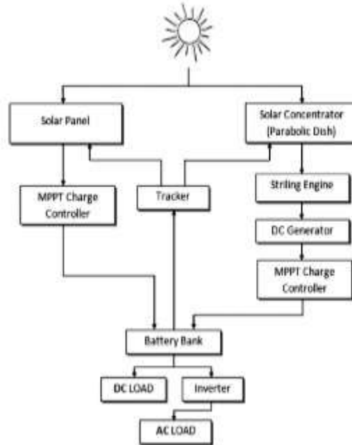
Fig 2.1 Block diagram of System
