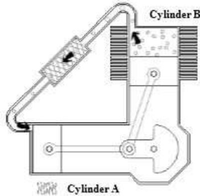
Fig 3.5 Gas expanding isochoric in A
